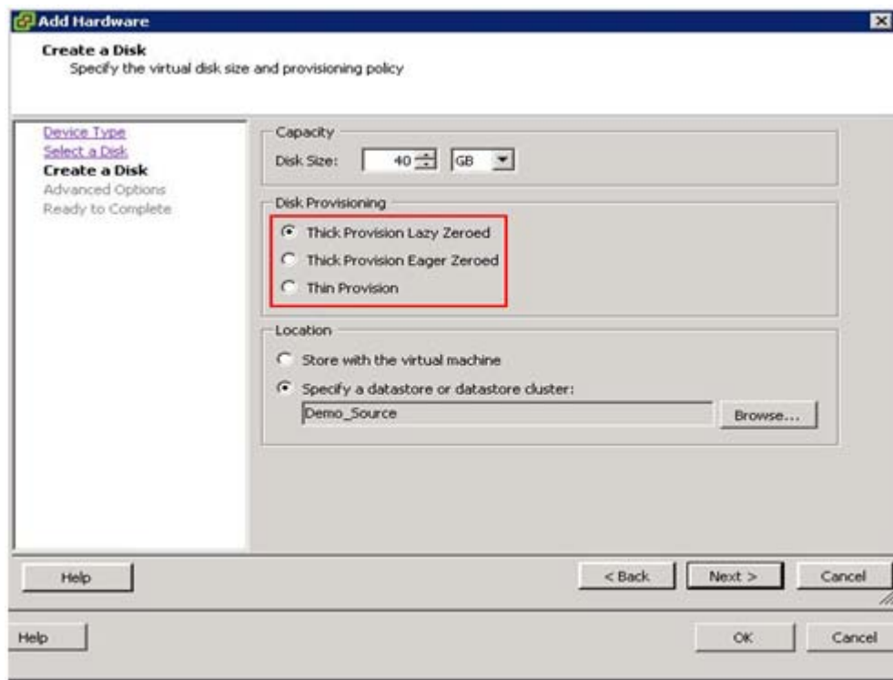
Figure 11. Disk Provisioning options with VAAI
