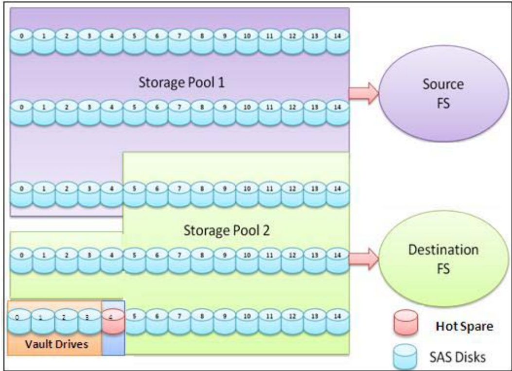
Figure 6. Storage architecture
