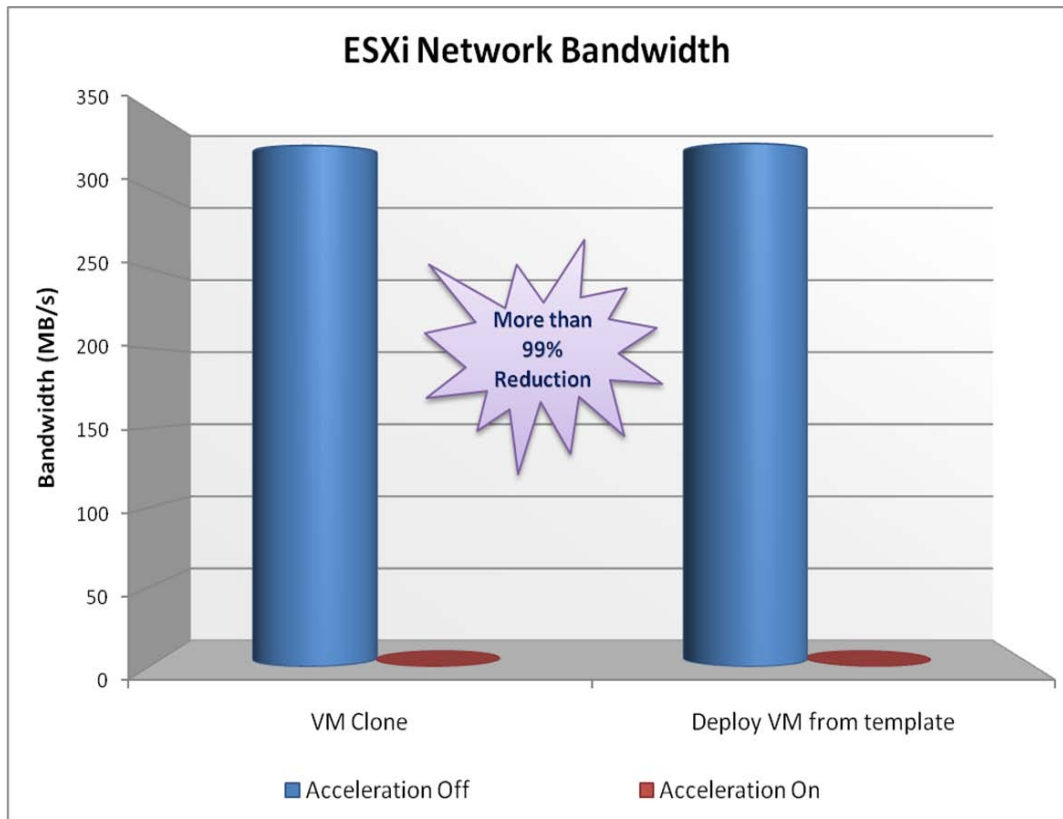
Figure 9. ESXi network utilization
