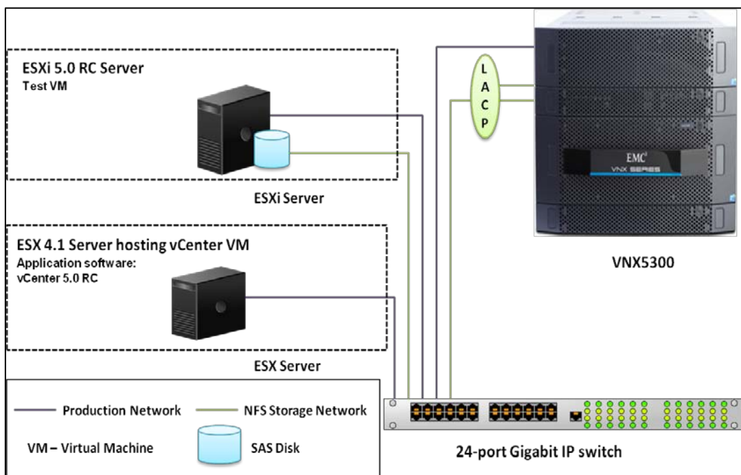
Figure 5. Reference architecture
