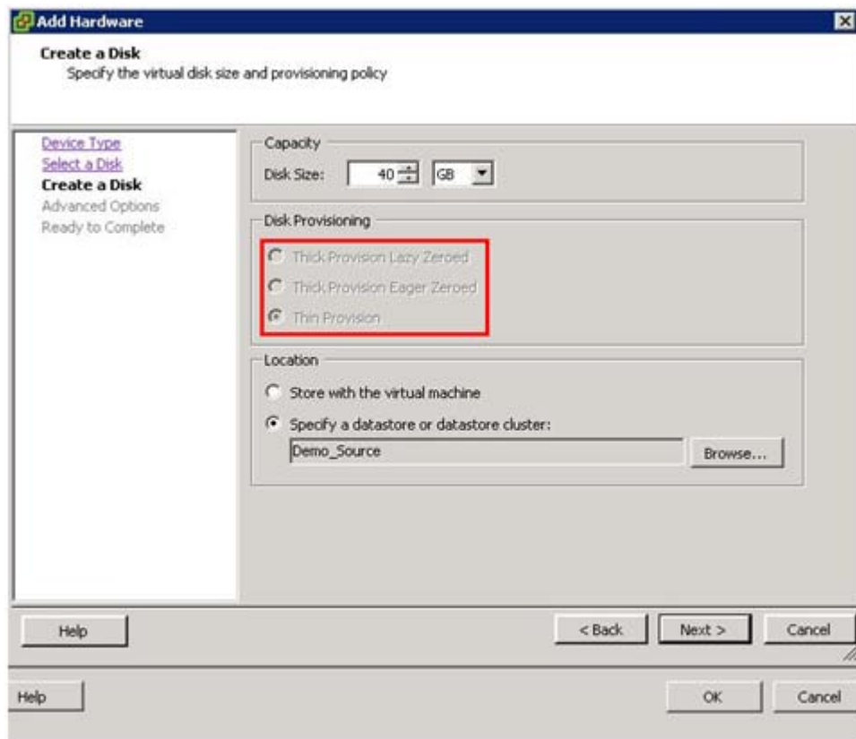
Figure 10. Disk Provisioning options on NFS datastores without VAAI support
