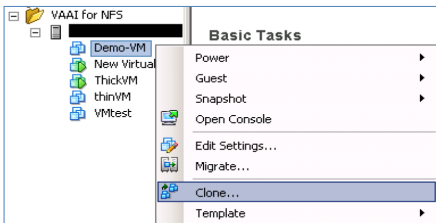
Figure 7. Initiate Full File Clone from vCenter Server
