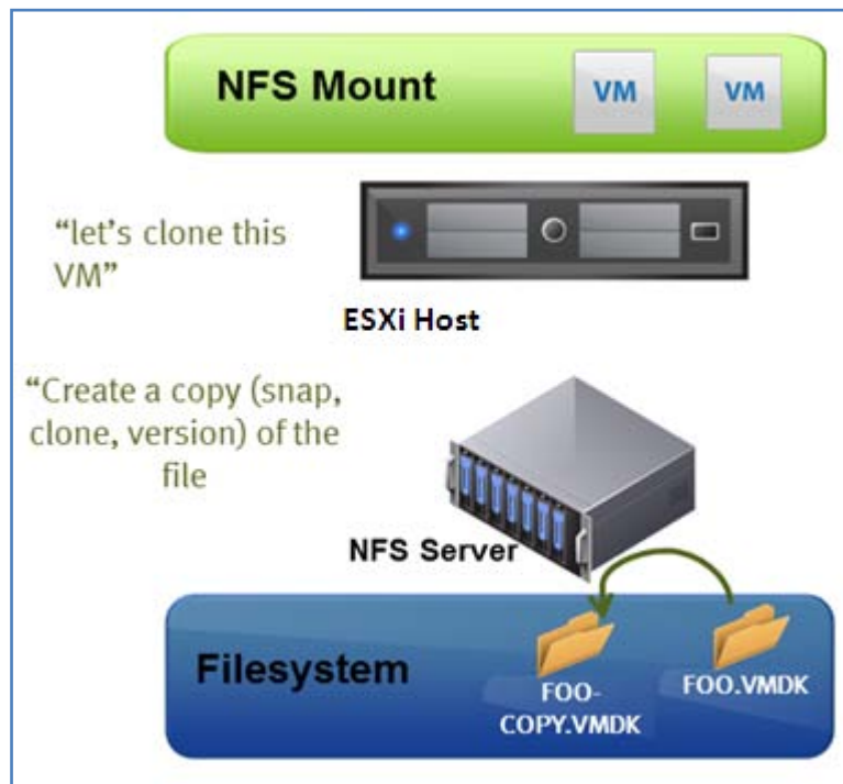
Figure 1. Full File Clones
